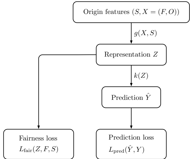
Figure 2: The framework of our method. The variables include sensitive attribute S , features X , outcome Y , representation Z , and prediction \hat{Y} . X is divided into fair variables F and other variables O . The function g maps the original features into the representation space, and function k maps the representations into the outcome space. There are two loss functions that measure utility and fairness respectively.
